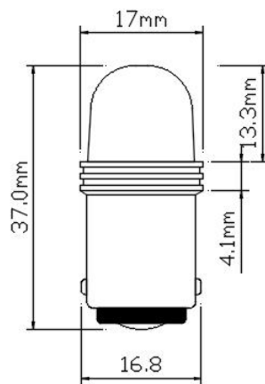
0° View
